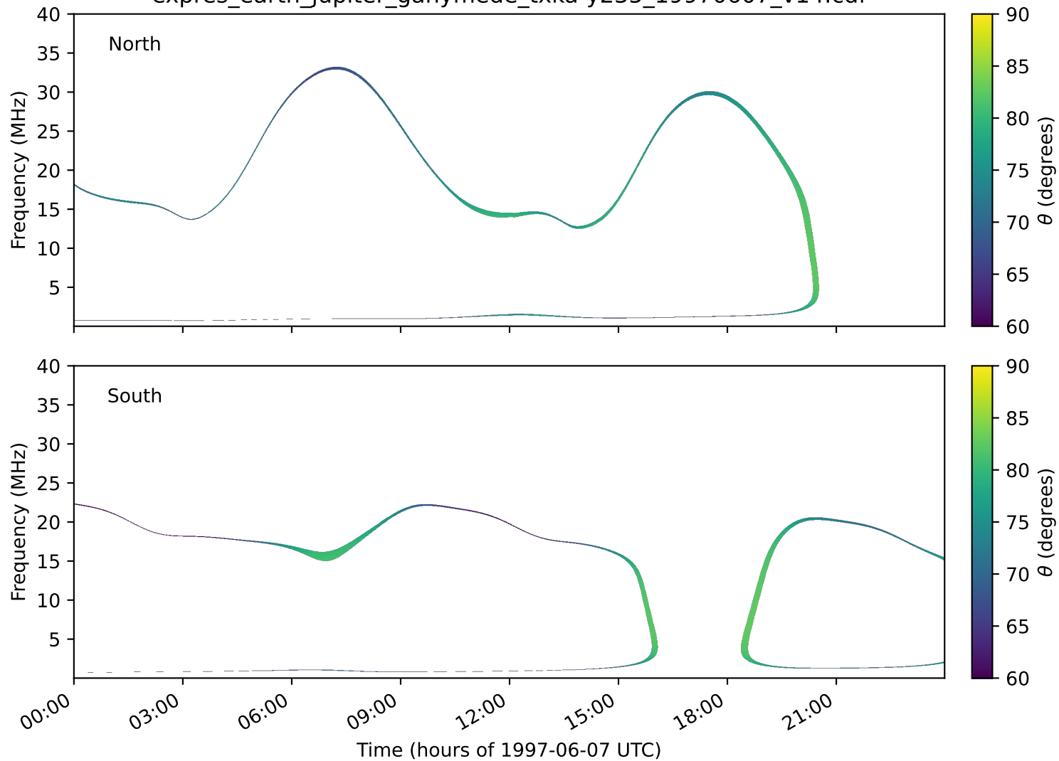
expres_earth_jupiter_ganymede_txka-y235_19970607_v14.cdf
