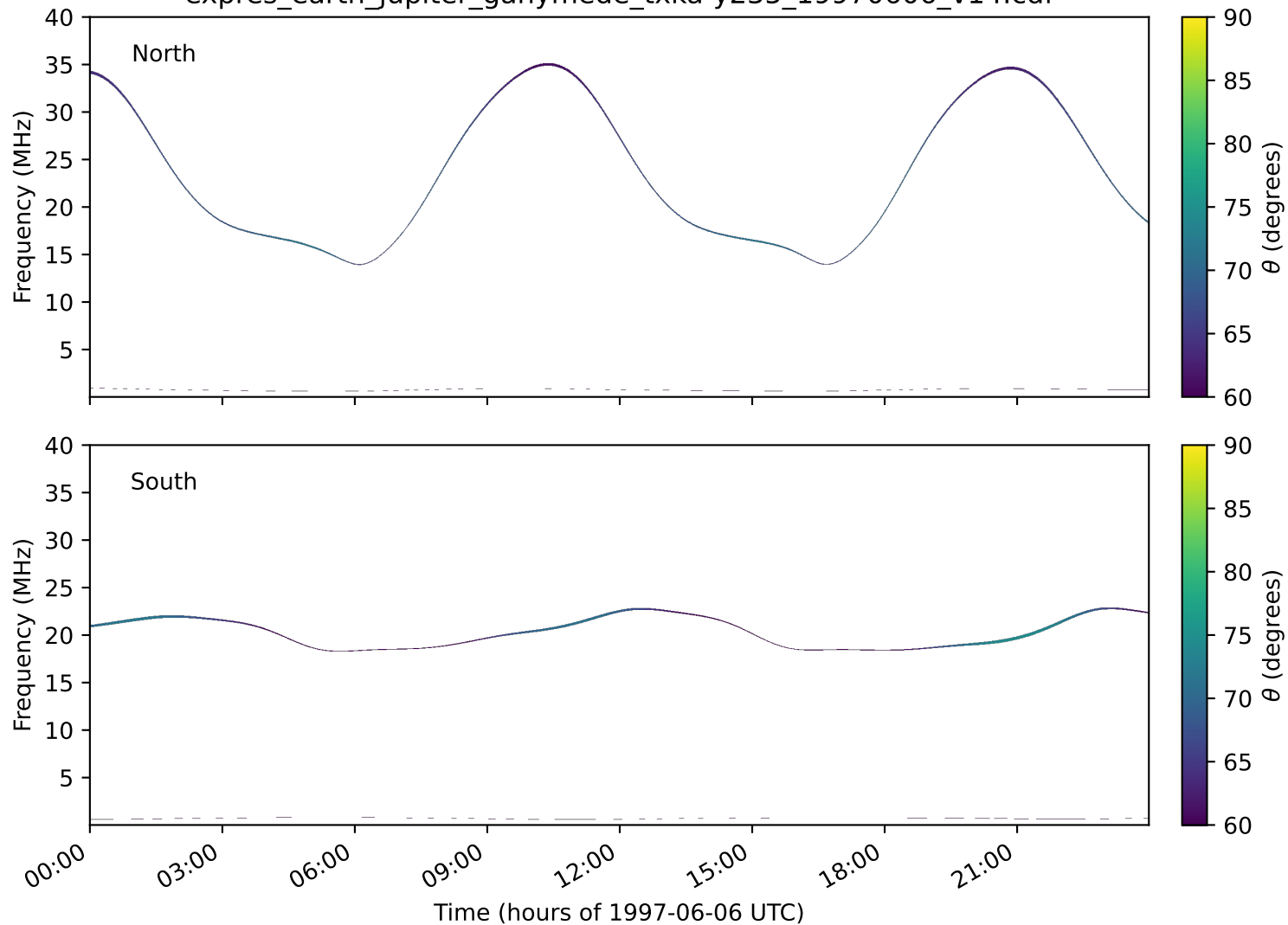
expres_earth_jupiter_ganymede_txka-y235_19970606_v14.cdf
