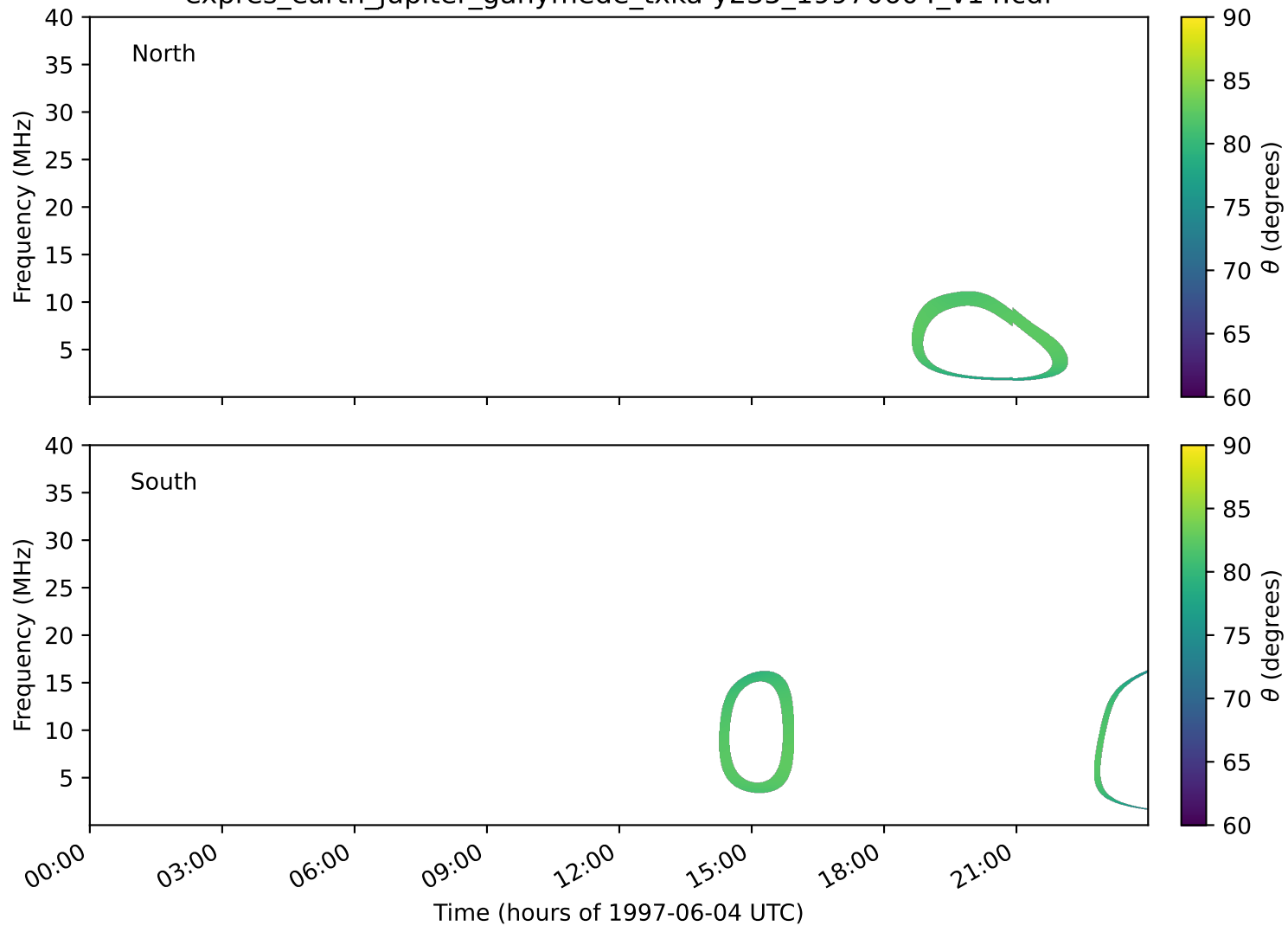
expres_earth_jupiter_ganymede_txka-y235_19970604_v14.cdf
