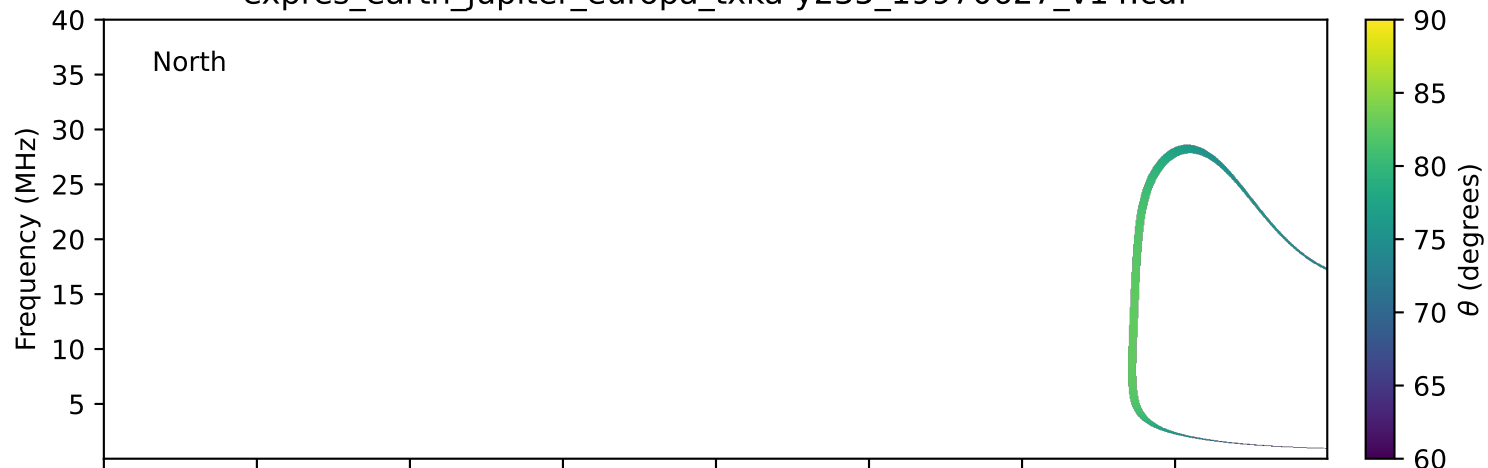
expres_earth_jupiter_europa_txka-y235_19970627_v14.cdf
