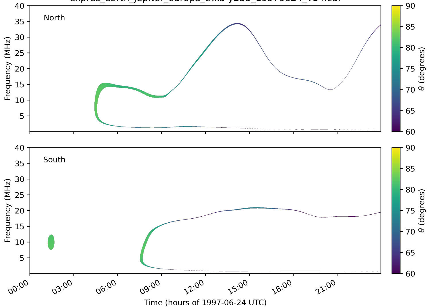
expres_earth_jupiter_europa_txka-y235_19970624_v14.cdf
