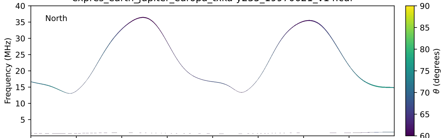
expres_earth_jupiter_europa_txka-y235_19970621_v14.cdf
