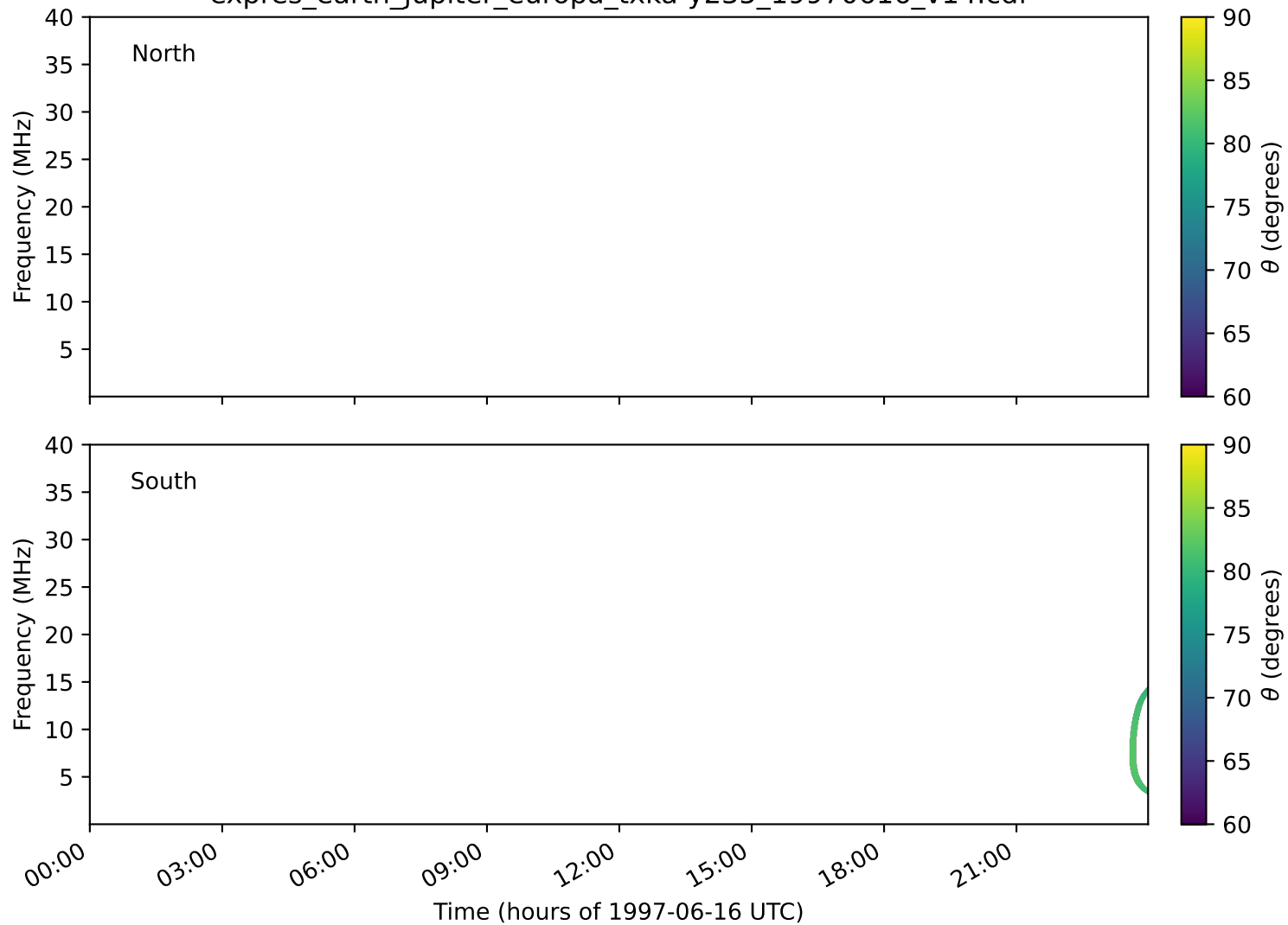
expres_earth_jupiter_europa_txka-y235_19970616_v14.cdf
