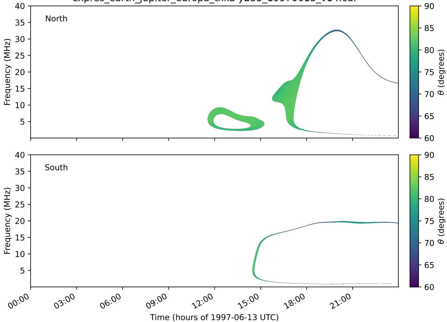
expres_earth_jupiter_europa_txka-y235_19970613_v14.cdf
