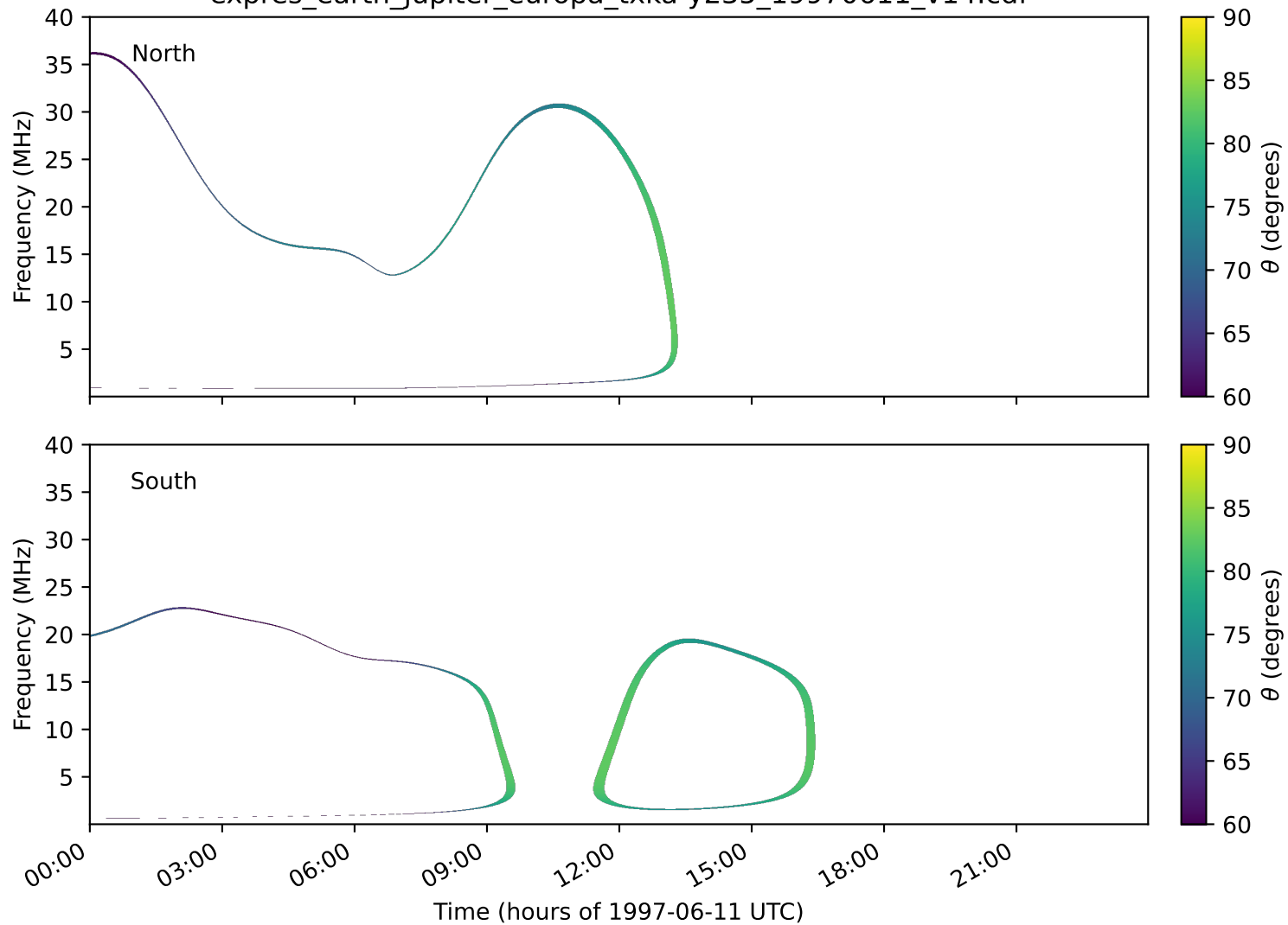
expres_earth_jupiter_europa_txka-y235_19970611_v14.cdf
