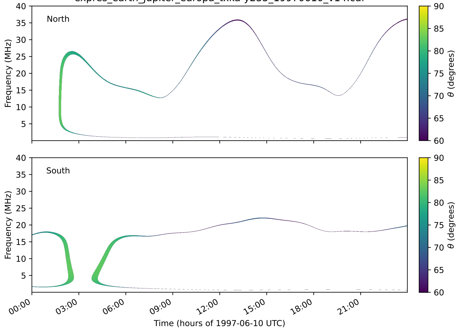
expres_earth_jupiter_europa_txka-y235_19970610_v14.cdf
