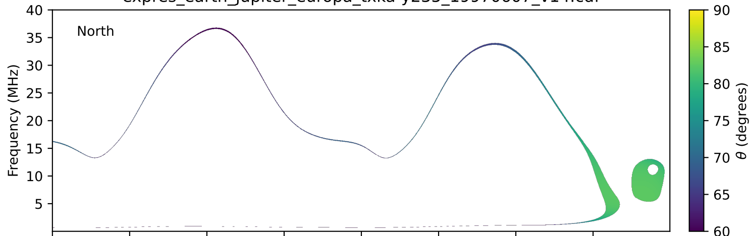
expres_earth_jupiter_europa_txka-y235_19970607_v14.cdf
