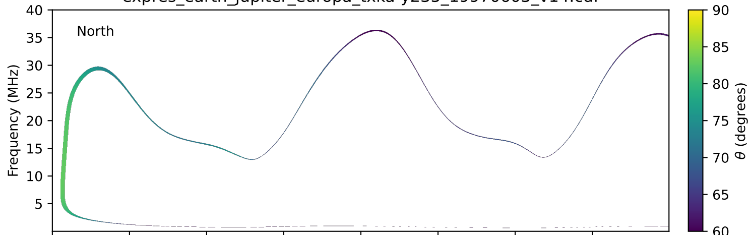
expres_earth_jupiter_europa_txka-y235_19970603_v14.cdf
