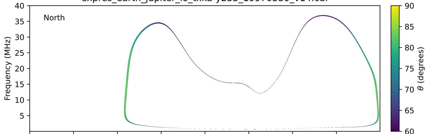
expres_earth_jupiter_io_txka-y235_19970530_v14.cdf
