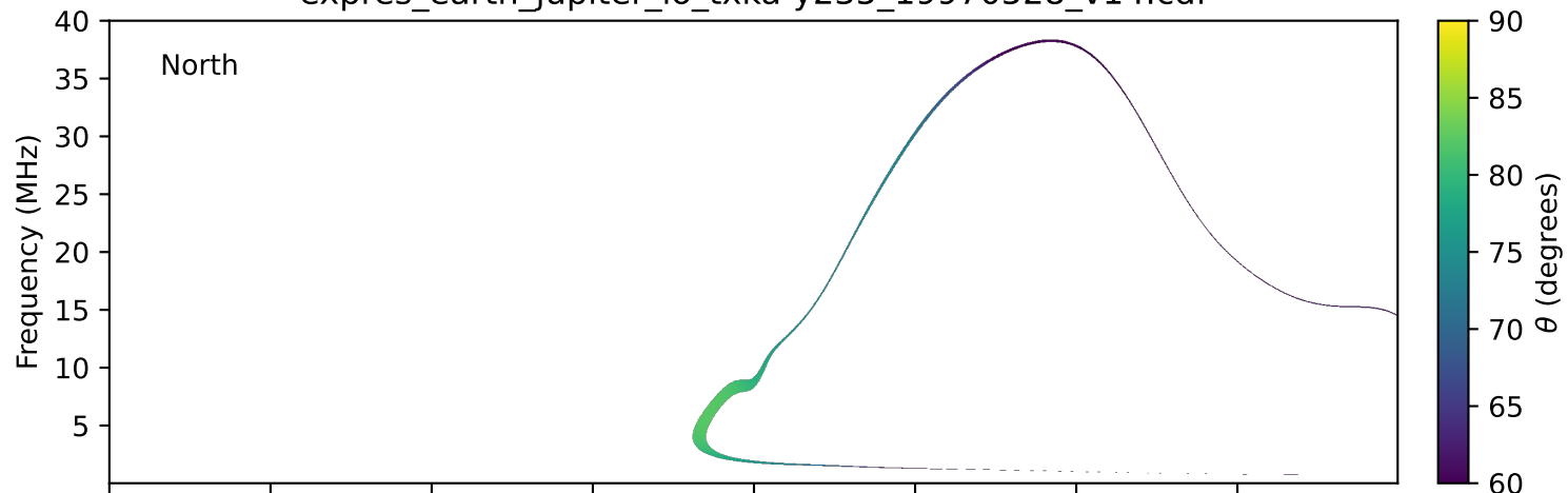
expres_earth_jupiter_io_txka-y235_19970528_v14.cdf
