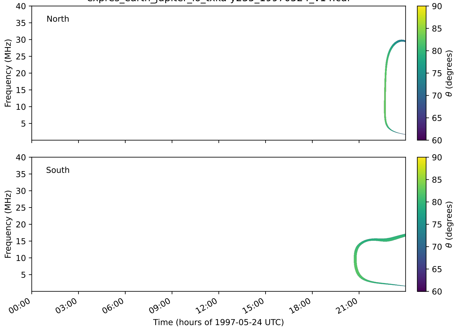
expres_earth_jupiter_io_txka-y235_19970524_v14.cdf
