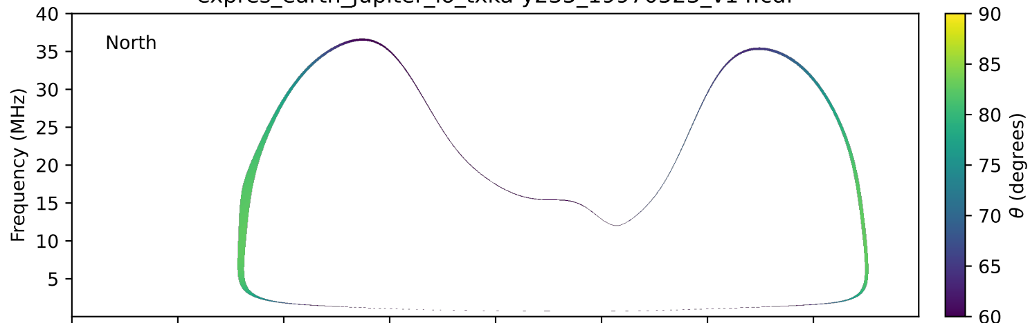
expres_earth_jupiter_io_txka-y235_19970523_v14.cdf
