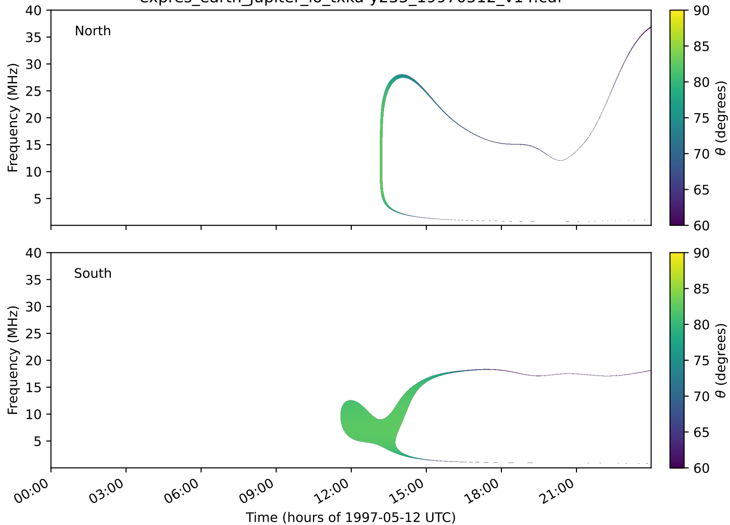
expres_earth_jupiter_io_txka-y235_19970512_v14.cdf
