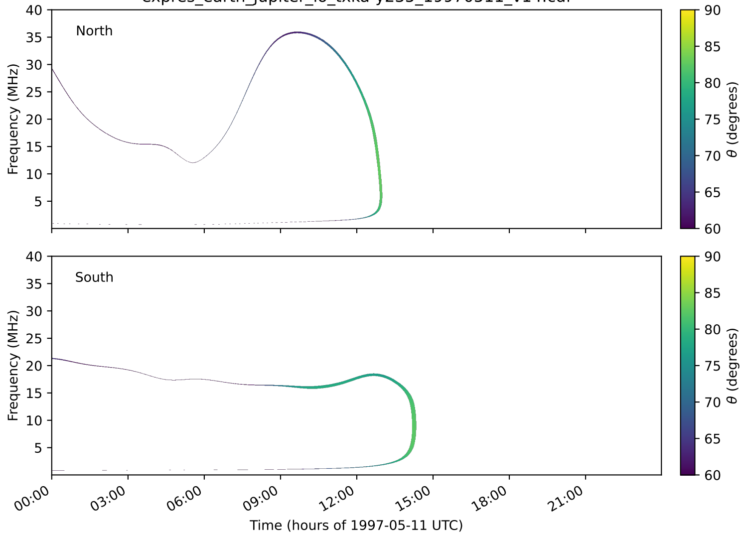
expres_earth_jupiter_io_txka-y235_19970511_v14.cdf
