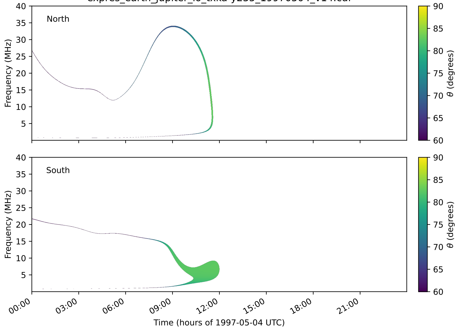
expres_earth_jupiter_io_txka-y235_19970504_v14.cdf
