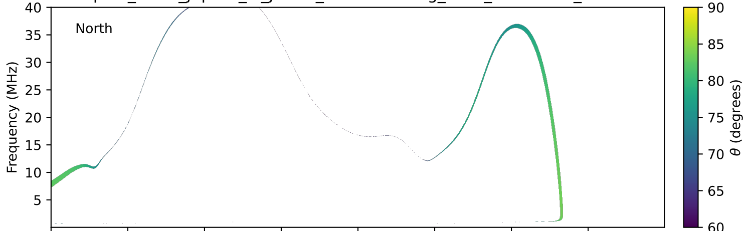
expres_earth_jupiter_io_jrm33_lossc-wid1deg_3kev_19970509_v11.cdf
