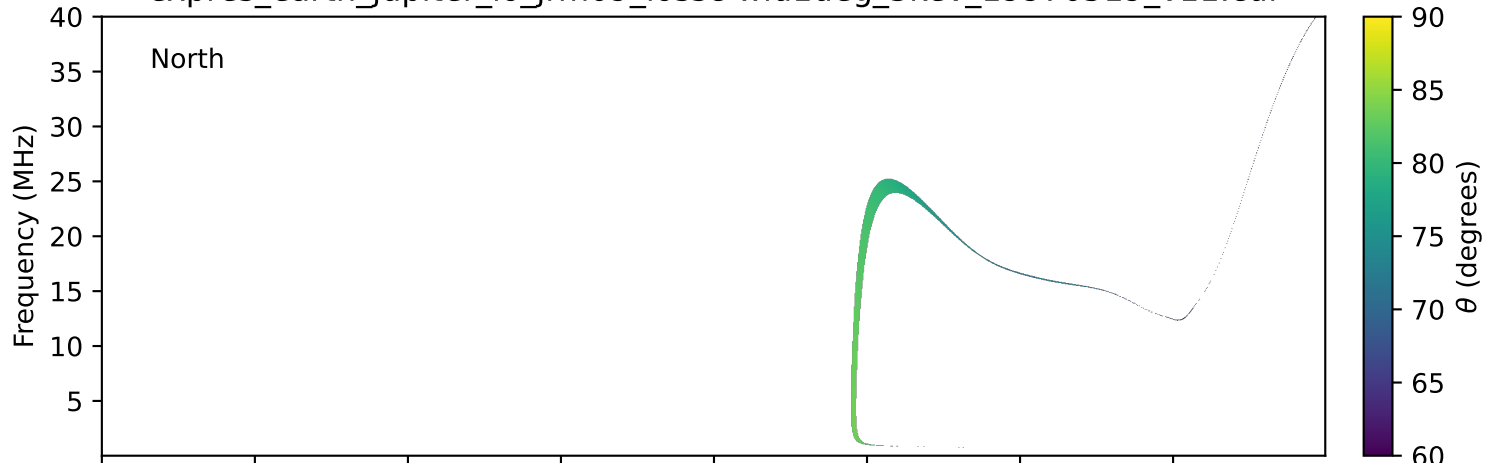
expres_earth_jupiter_io_jrm09_lossc-wid1deg_3kev_19970519_v11.cdf
