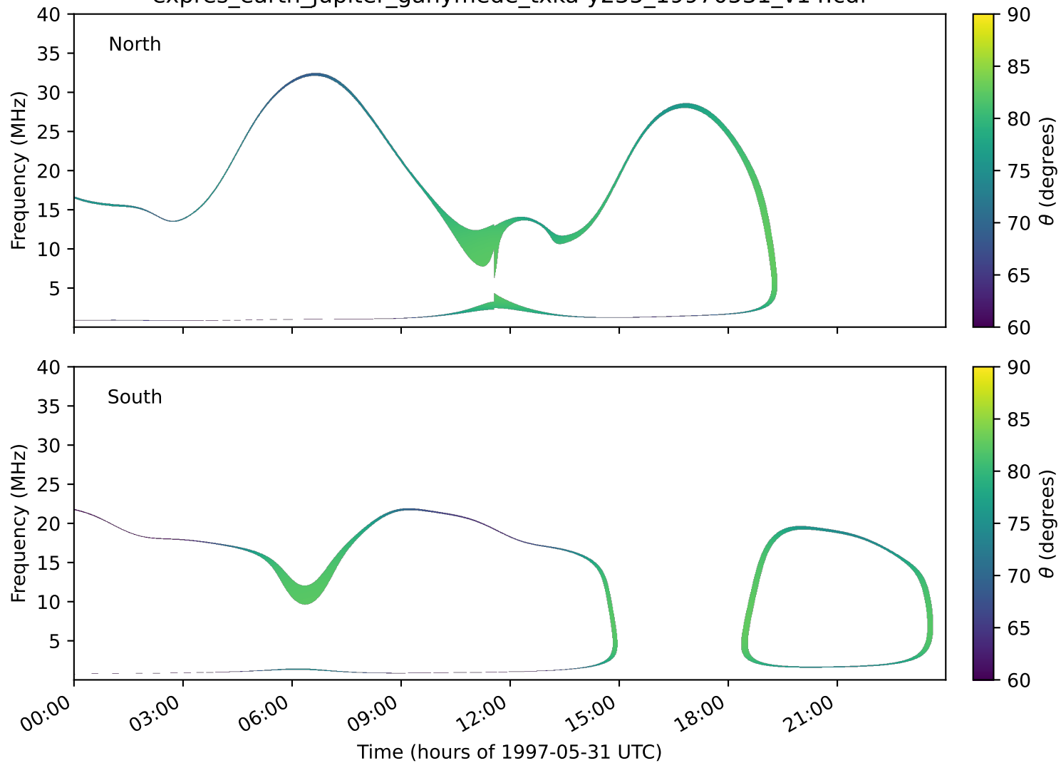
expres_earth_jupiter_ganymede_txka-y235_19970531_v14.cdf
