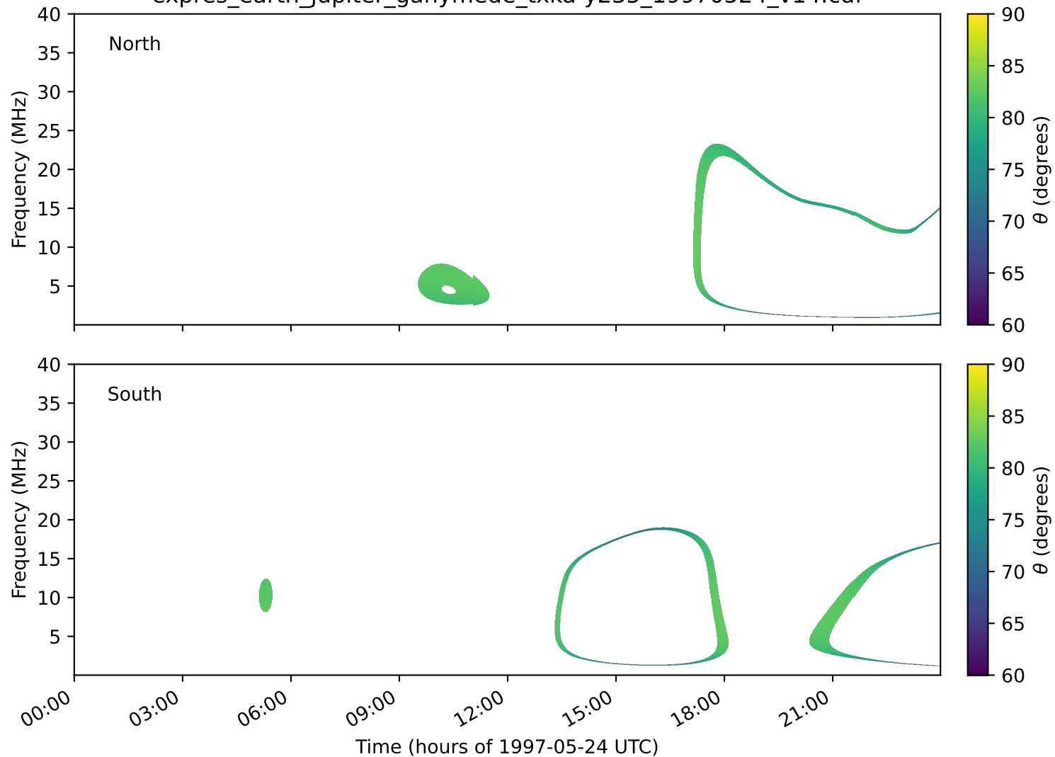
expres_earth_jupiter_ganymede_txka-y235_19970524_v14.cdf
