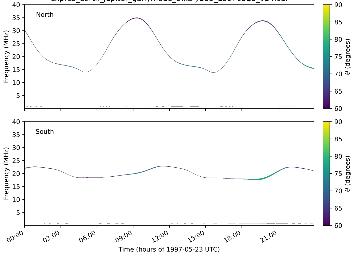
expres_earth_jupiter_ganymede_txka-y235_19970523_v14.cdf
