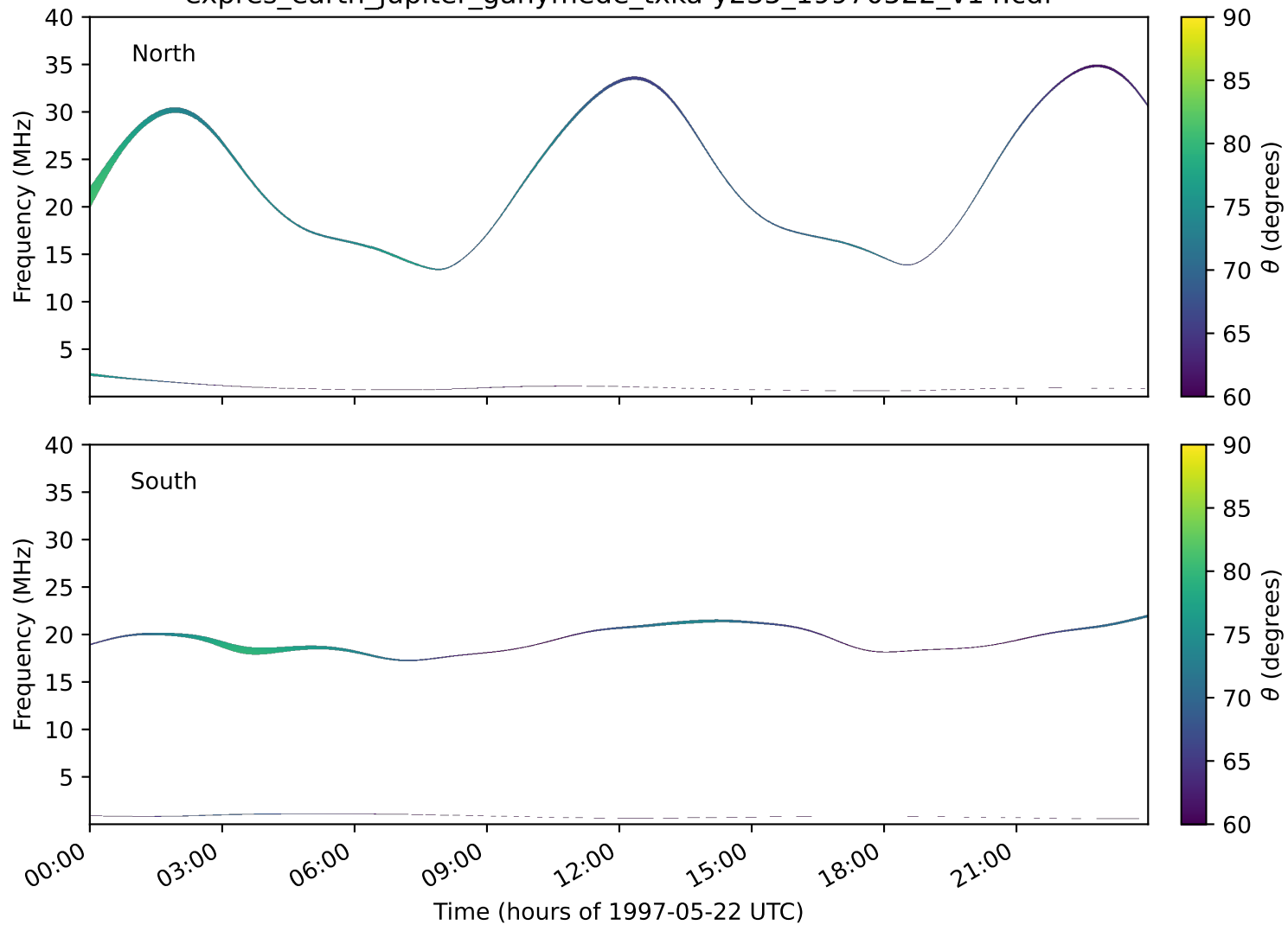
expres_earth_jupiter_ganymede_txka-y235_19970522_v14.cdf
