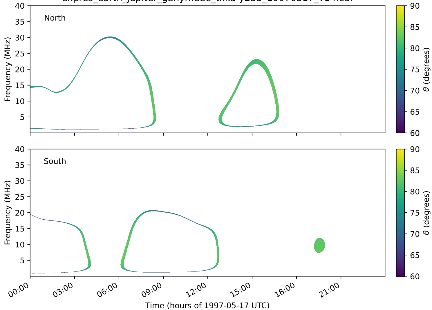
expres_earth_jupiter_ganymede_txka-y235_19970517_v14.cdf
