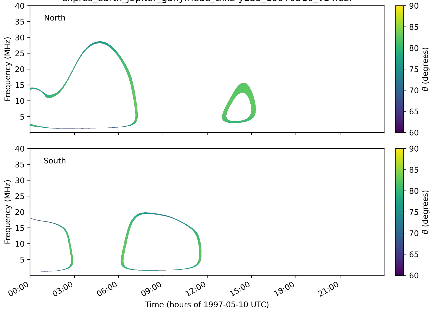
expres_earth_jupiter_ganymede_txka-y235_19970510_v14.cdf
