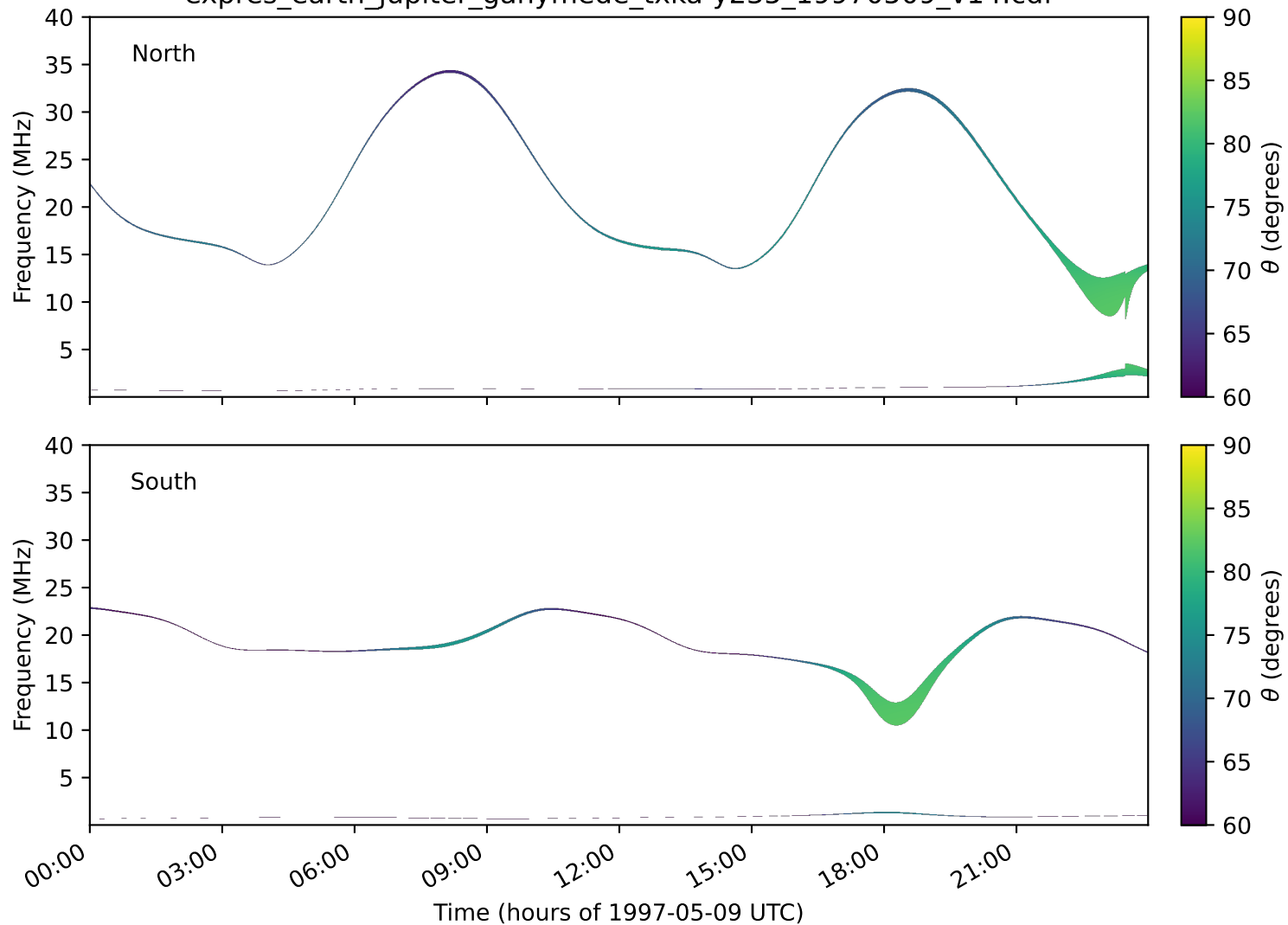
expres_earth_jupiter_ganymede_txka-y235_19970509_v14.cdf
