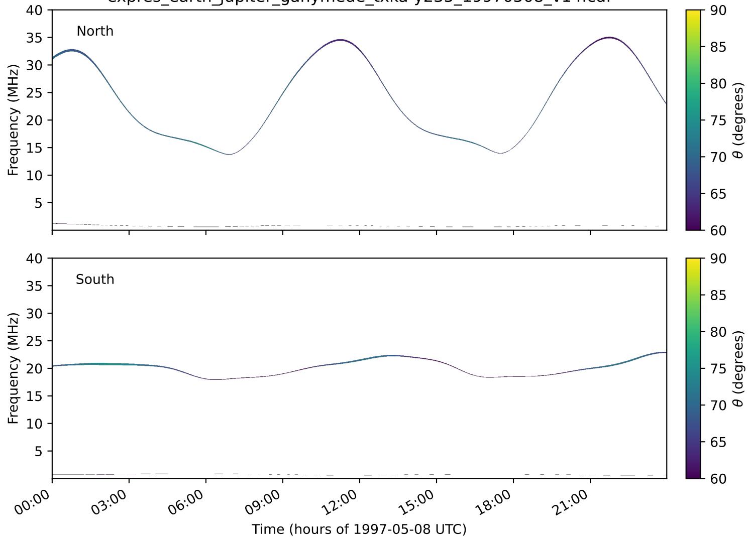
expres_earth_jupiter_ganymede_txka-y235_19970508_v14.cdf
