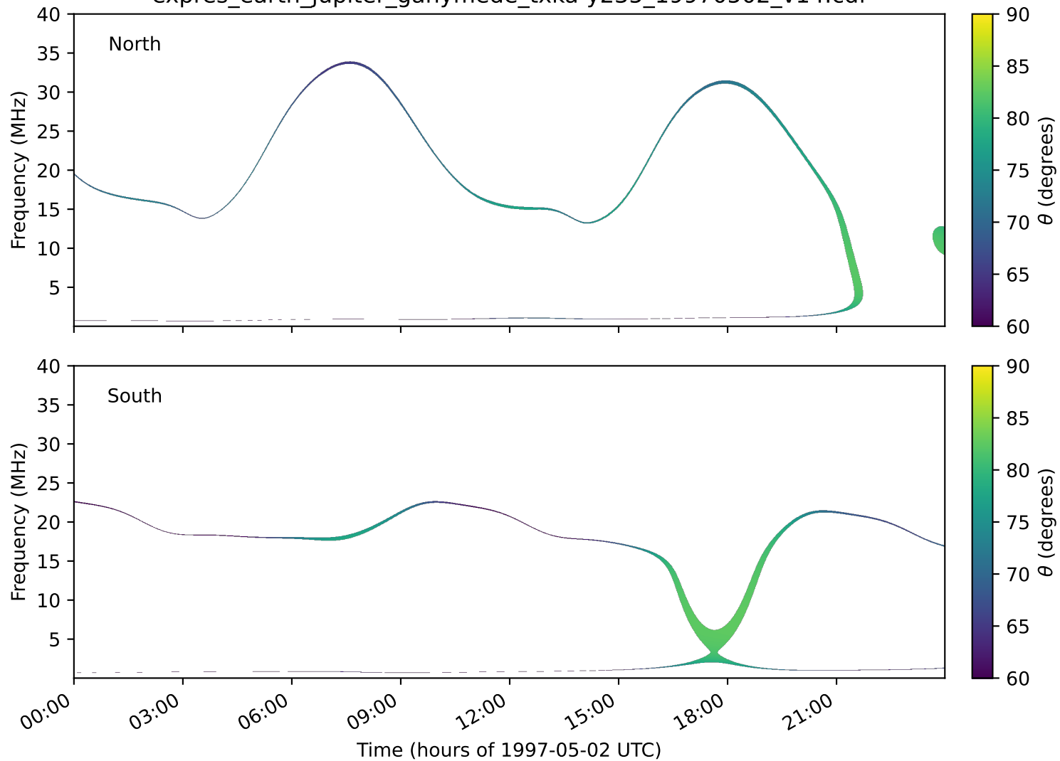
expres_earth_jupiter_ganymede_txka-y235_19970502_v14.cdf
