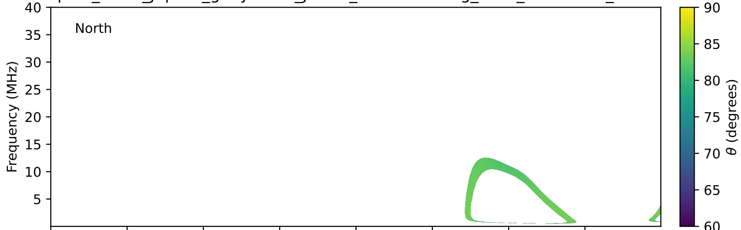
expres_earth_jupiter_ganymede_jrm33_lossc-wid1deg_3kev_19970521_v11.cdf
