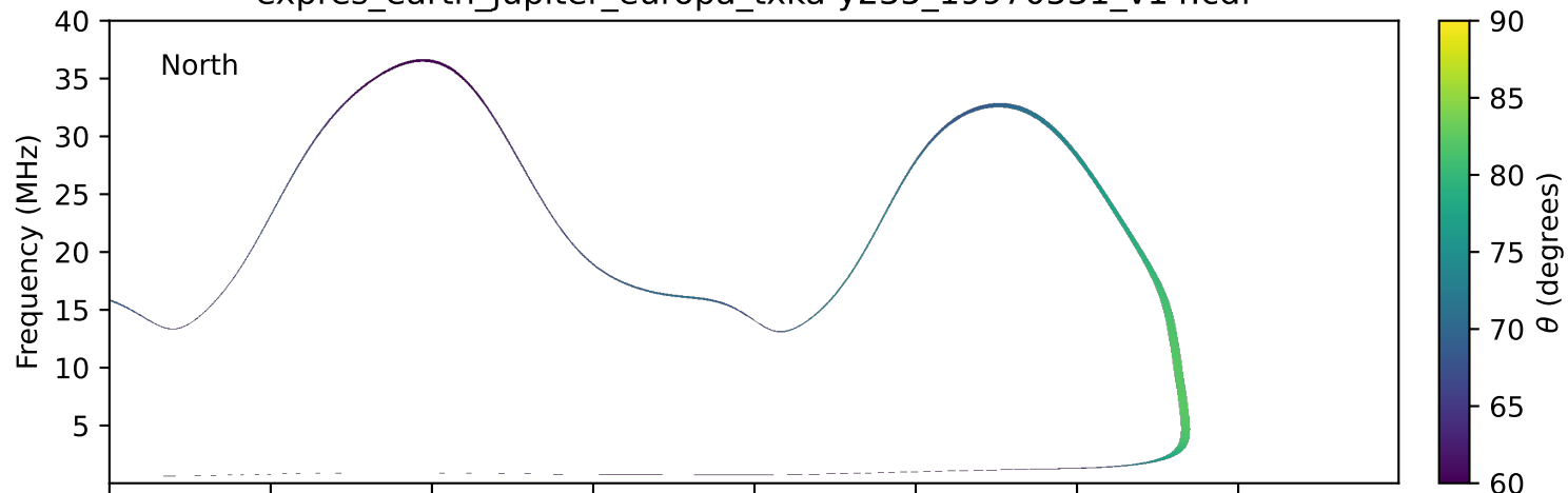
expres_earth_jupiter_europa_txka-y235_19970531_v14.cdf
