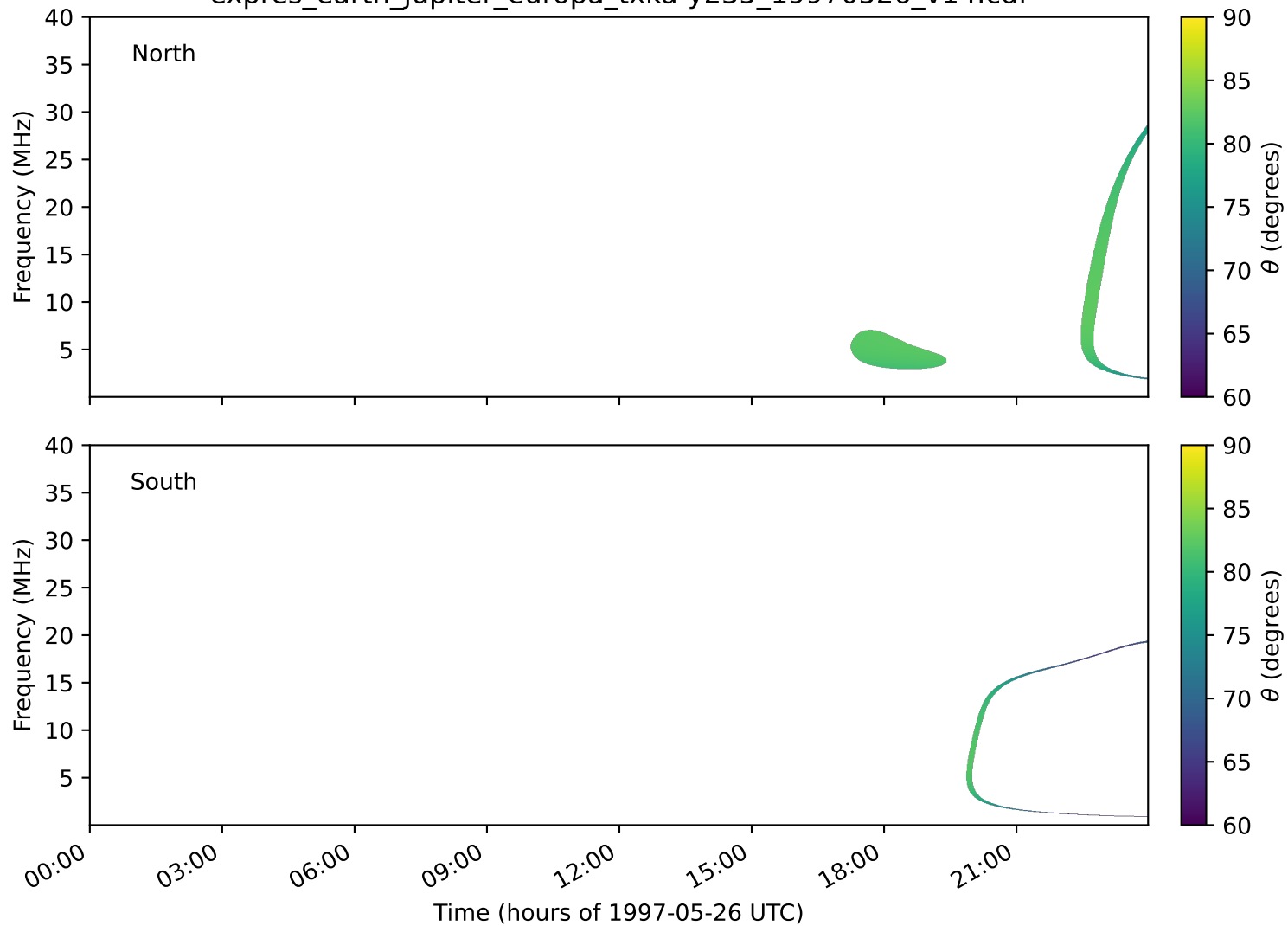
expres_earth_jupiter_europa_txka-y235_19970526_v14.cdf
