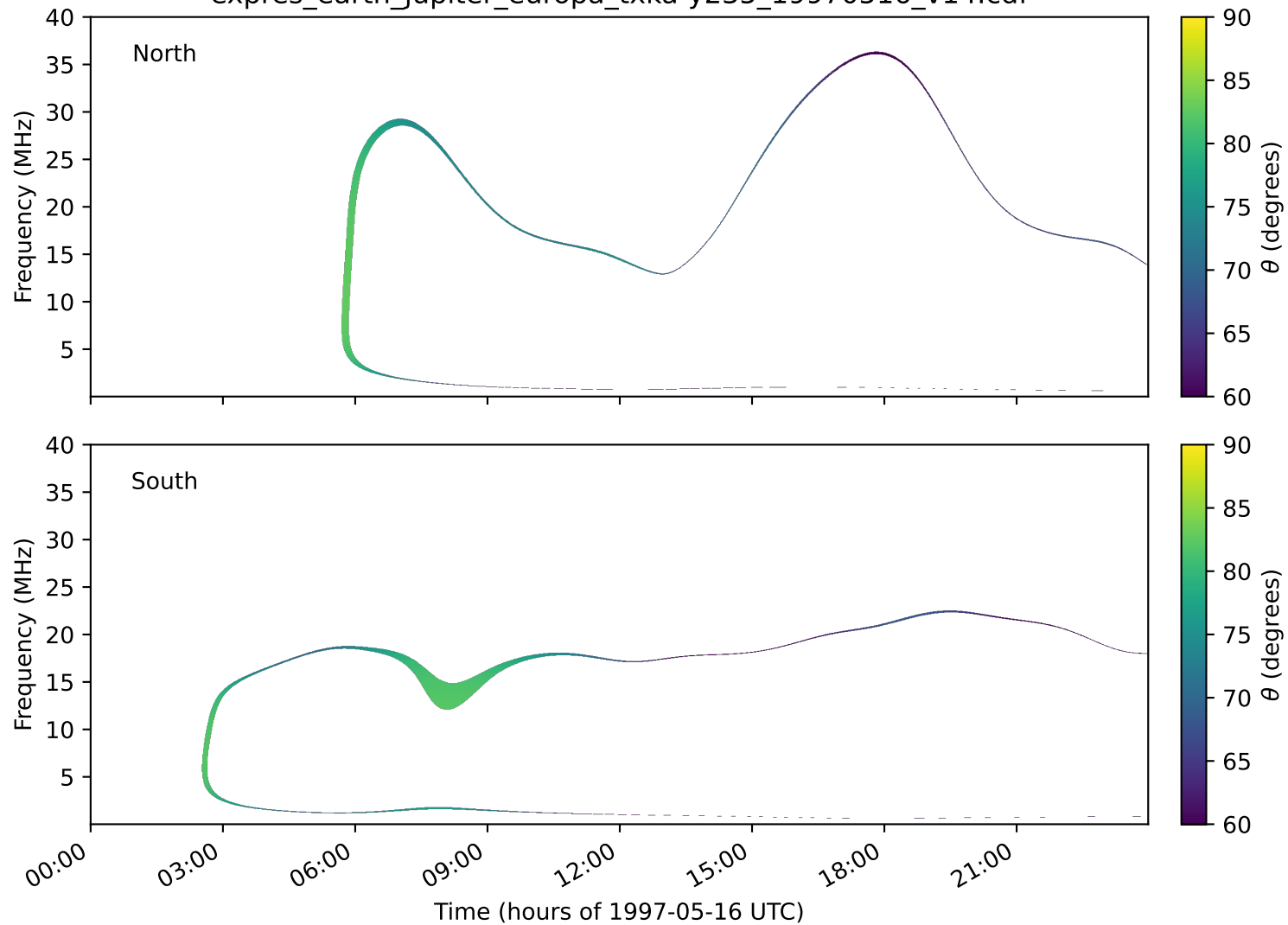
expres_earth_jupiter_europa_txka-y235_19970516_v14.cdf
