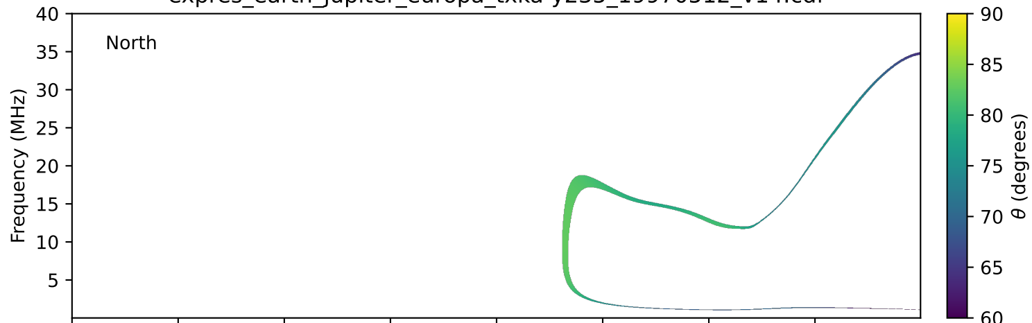
expres_earth_jupiter_europa_txka-y235_19970512_v14.cdf
