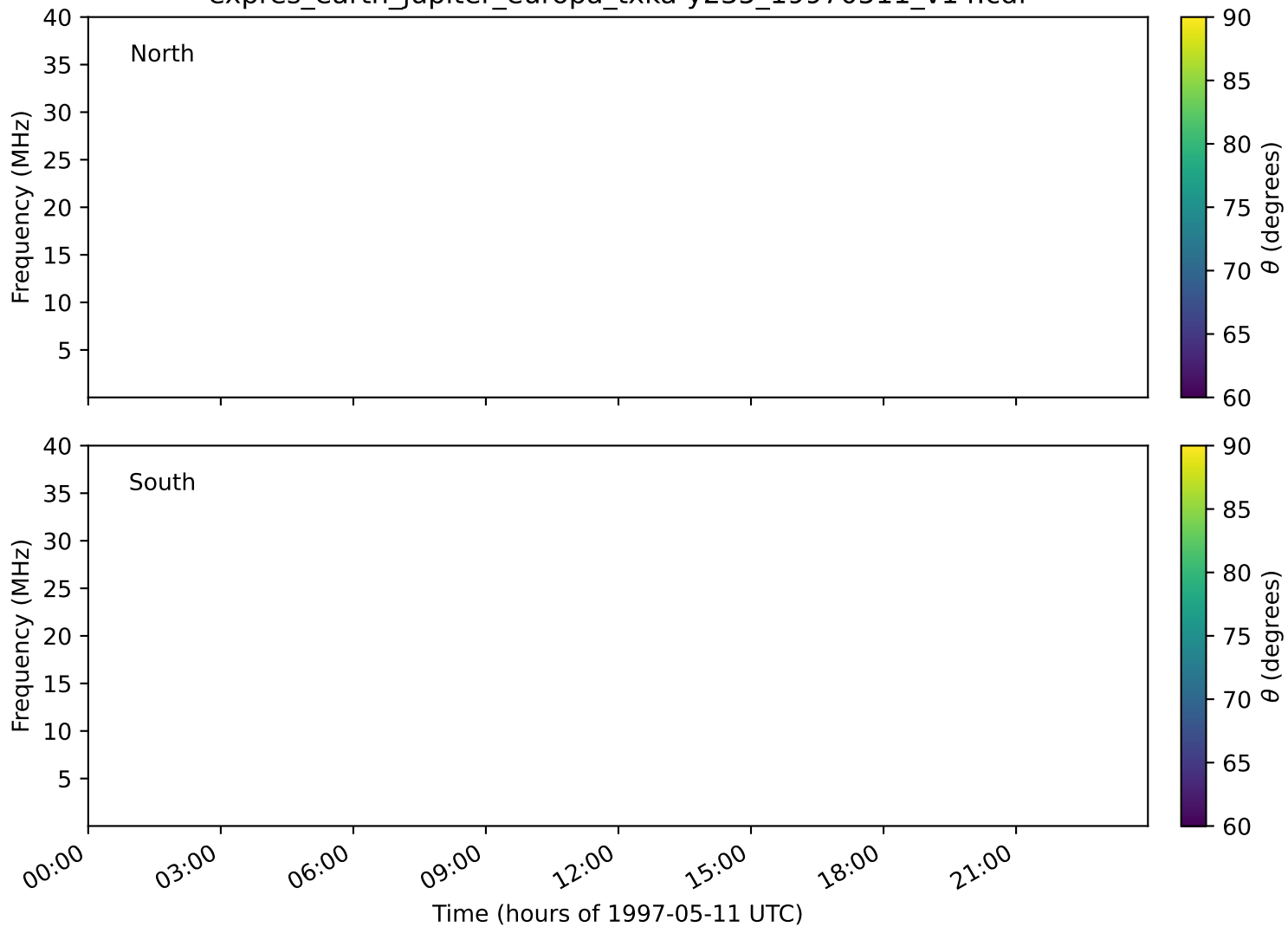
expres_earth_jupiter_europa_txka-y235_19970511_v14.cdf
