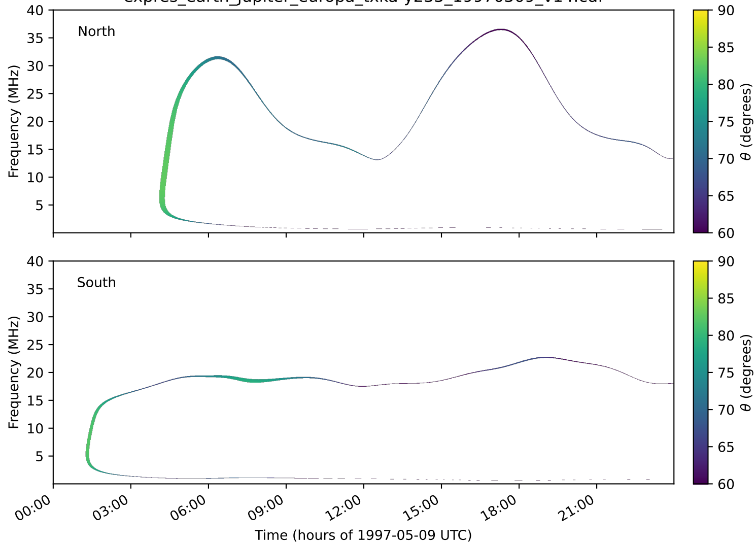
expres_earth_jupiter_europa_txka-y235_19970509_v14.cdf
