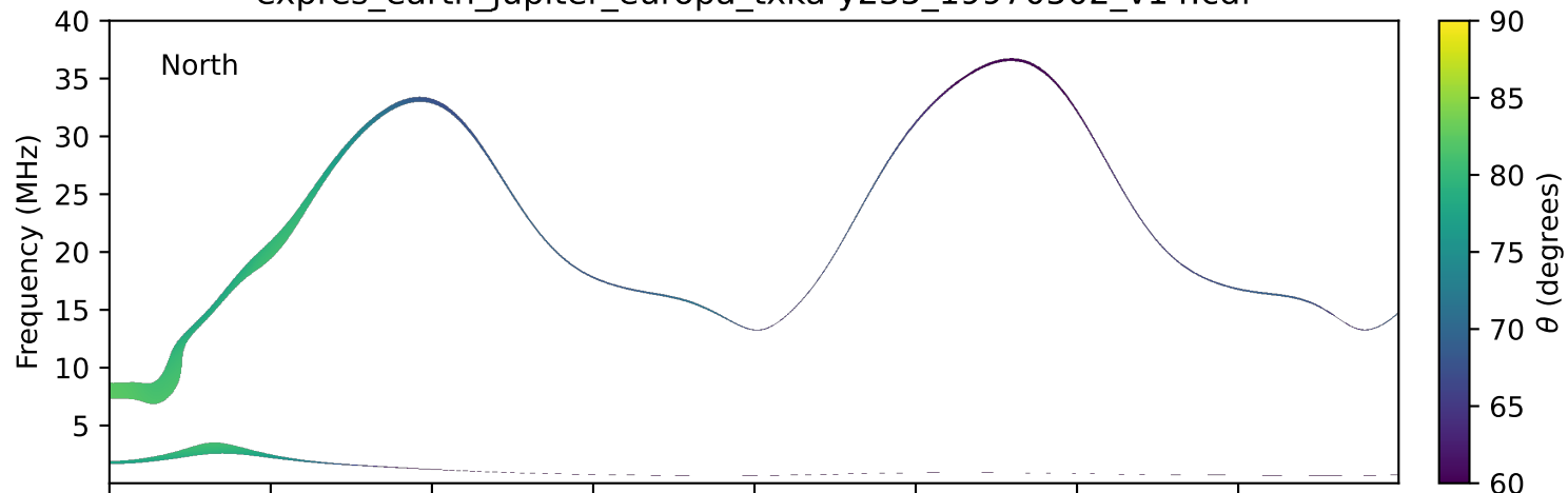
expres_earth_jupiter_europa_txka-y235_19970502_v14.cdf
