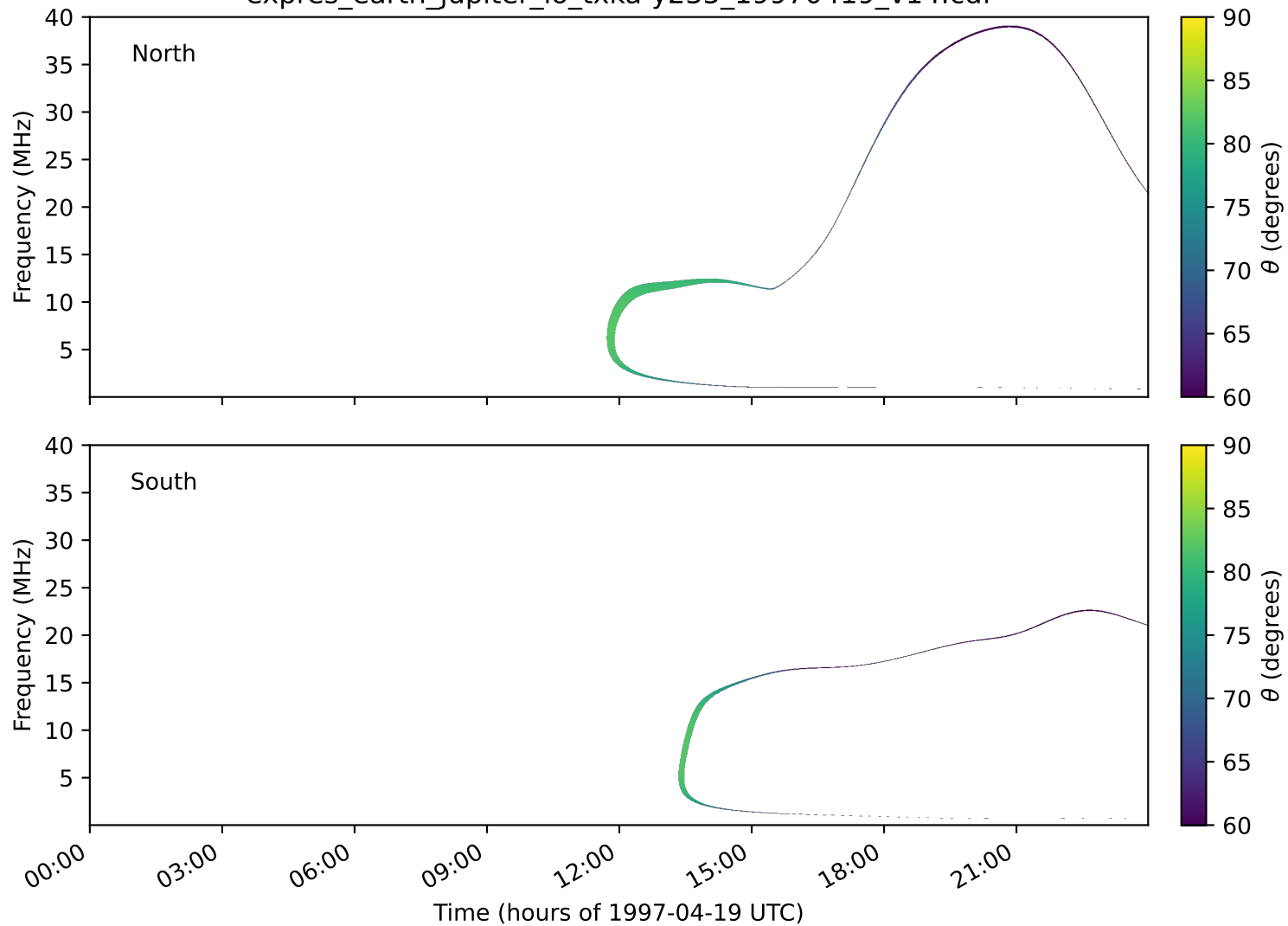
expres_earth_jupiter_io_txka-y235_19970419_v14.cdf
