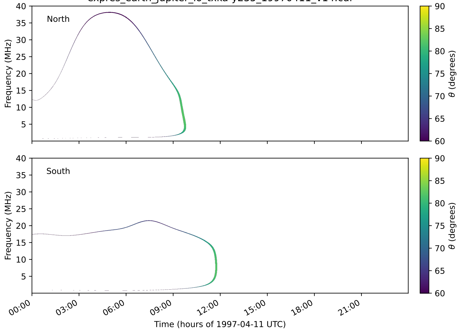
expres_earth_jupiter_io_txka-y235_19970411_v14.cdf
