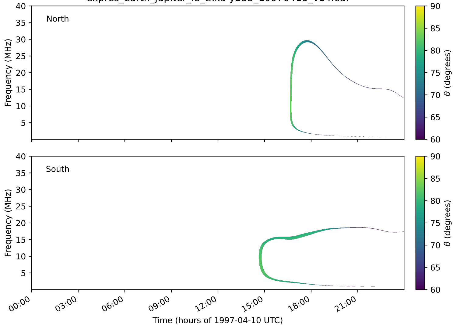
expres_earth_jupiter_io_txka-y235_19970410_v14.cdf
