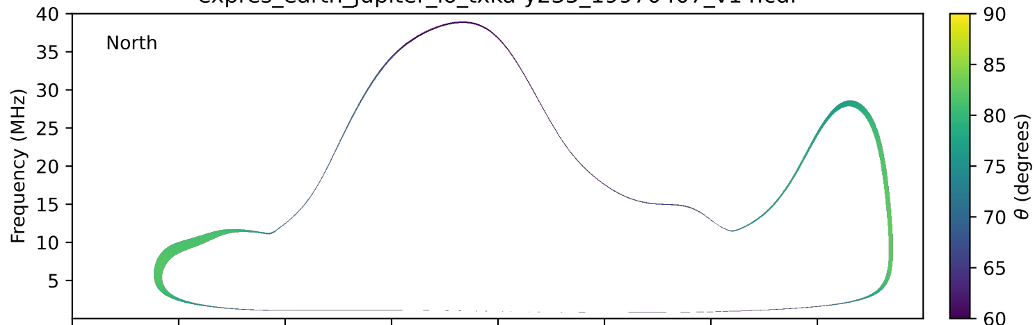
expres_earth_jupiter_io_txka-y235_19970407_v14.cdf
