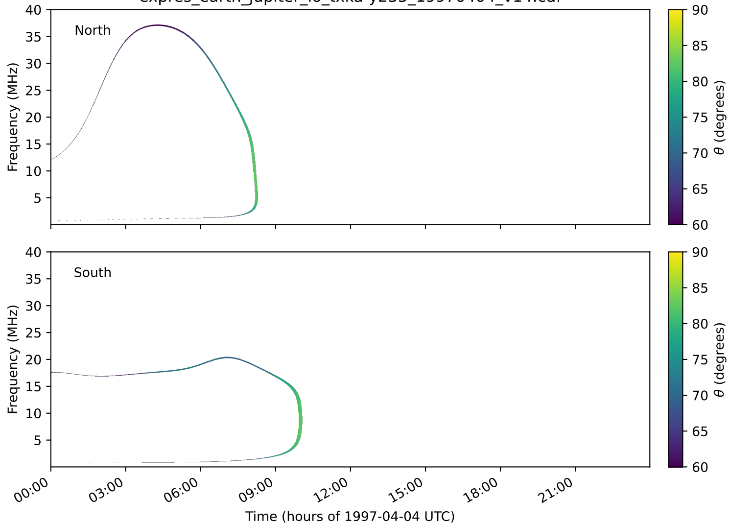
expres_earth_jupiter_io_txka-y235_19970404_v14.cdf
