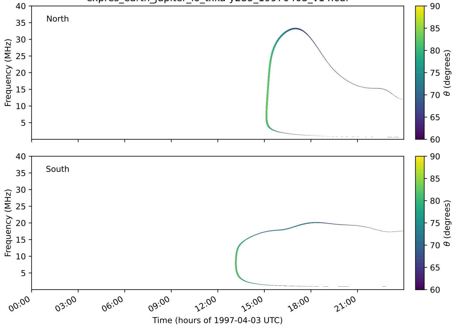
expres_earth_jupiter_io_txka-y235_19970403_v14.cdf
