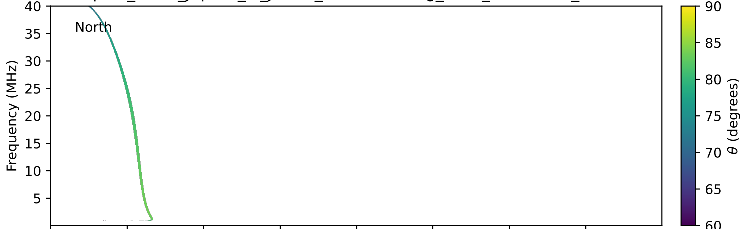
expres_earth_jupiter_io_jrm33_lossc-wid1deg_3kev_19970429_v11.cdf
