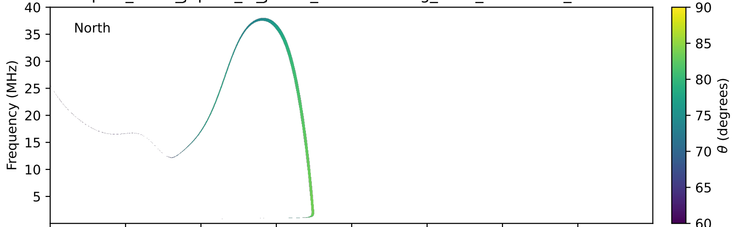
expres_earth_jupiter_io_jrm33_lossc-wid1deg_3kev_19970427_v11.cdf
