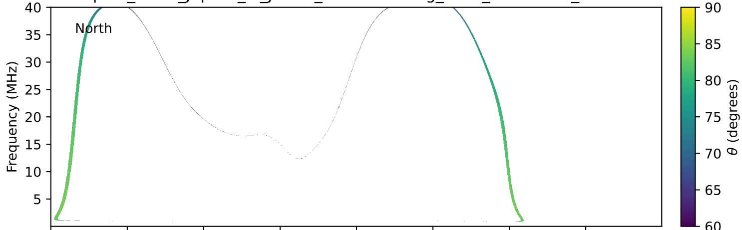
expres_earth_jupiter_io_jrm33_lossc-wid1deg_3kev_19970416_v11.cdf
