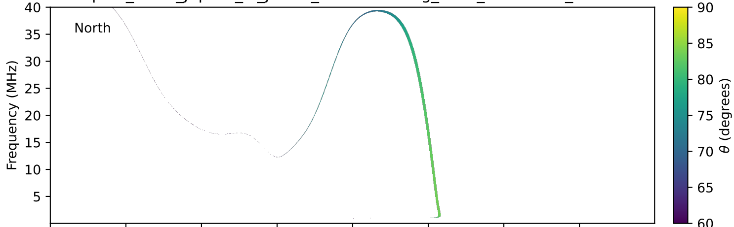
expres_earth_jupiter_io_jrm33_lossc-wid1deg_3kev_19970402_v11.cdf
