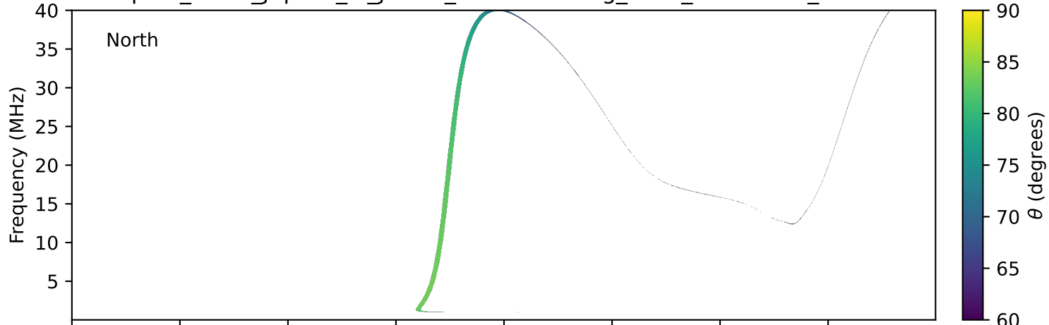
expres_earth_jupiter_io_jrm09_lossc-wid1deg_3kev_19970428_v11.cdf
