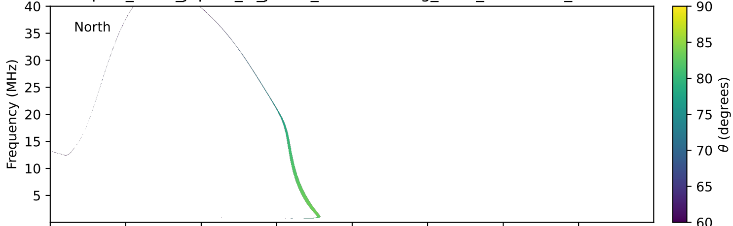
expres_earth_jupiter_io_jrm09_lossc-wid1deg_3kev_19970411_v11.cdf
